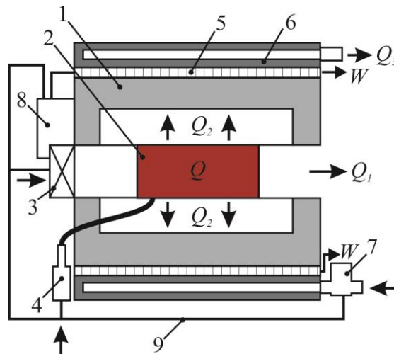
Fig. 3. Physical model of "starting pre-heater – thermoelectric generator" system
